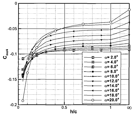
Fig. 13 Moment coefficient at quarter chord vs. h/c for each angle of attack
