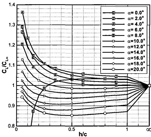
Fig. 9 Lift coefficient variation by the ground effect
