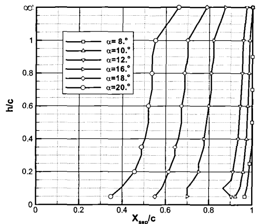
Fig. 16 Separation point vs. h/c for each alpha
