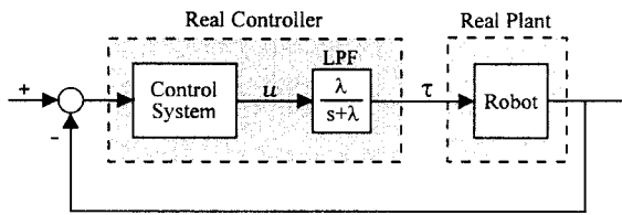
Fig. 2. Block Diagram of the Real System
