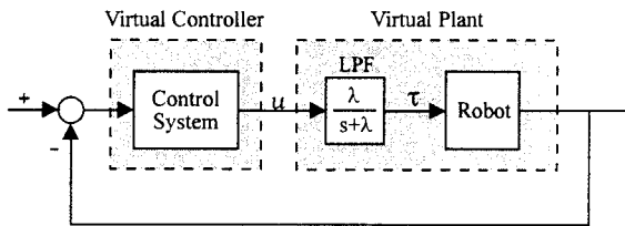
Fig. 1. Block Diagram of the Virtual System
