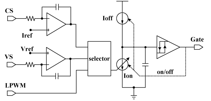
Fig. 4. Simplified block diagram of the control circuits.
