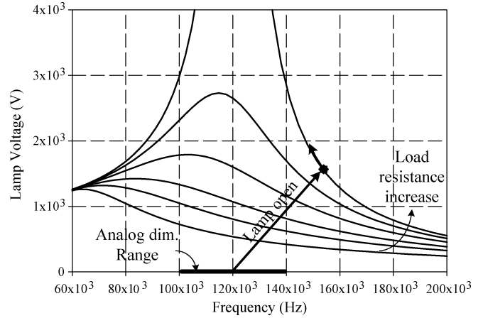
Fig. 6. Simulated frequency characteristics of the lamp's voltage.
