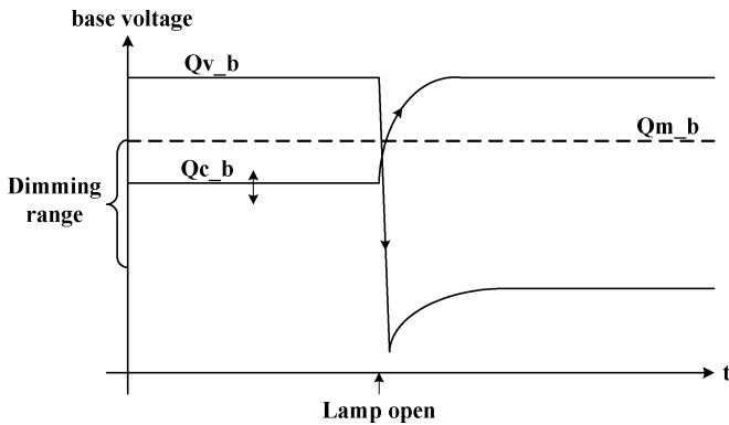
Fig. 7. Representative base voltages for lamp open.
