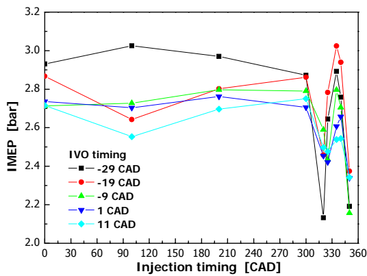
Figure 9 IMEP of LPG-DME CI engine with respect to injection timing and intake valve open timing at 1000rpm
