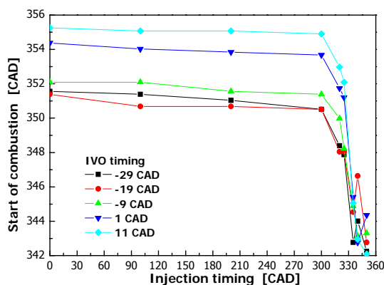
Figure 10 start of combustion timing of LPG-DME CI engine with respect to injection timing and intake valve open timing at 1000rpm
