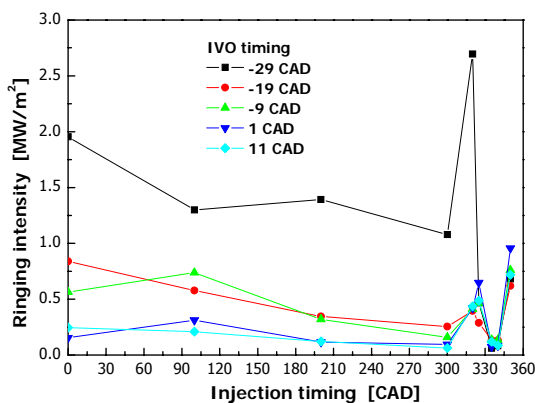
Figure 14 Ringing intensity of LPG-DME CI engine with respect to injection timing and intake valve open timing at 1000rpm
