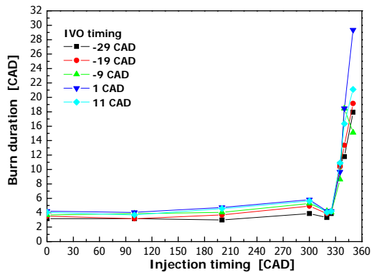
Figure 13 burn duration of LPG-DME CI engine with respect to injection timing and intake valve open timing at 1000rpm
