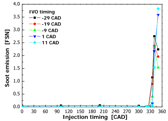
Figure 11 Soot emission of LPG-DME CI engine with respect to injection timing and intake valve open timing at 1000rpm
