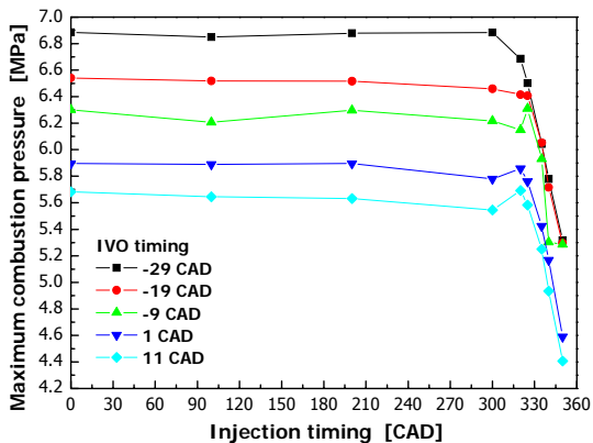
Figure 15 Maximum combustion pressure of LPG-DME CI engine with respect to injection timing and intake valve open timing at 1000rpm
