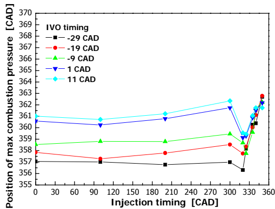
Figure 16 Position of maximum combustion pressure of LPG-DME CI engine with respect to injection timing and intake valve open timing at 1000rpm
