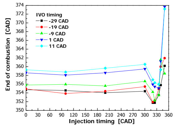
Figure 12 end of combustion timing of LPG-DME CI engine with respect to injection timing and intake valve open timing at 1000rpm
