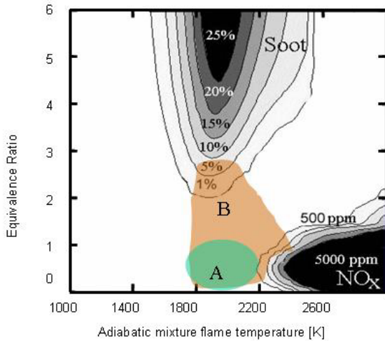
Figure 8 The soot and NOx formation in \phi -T diagram
