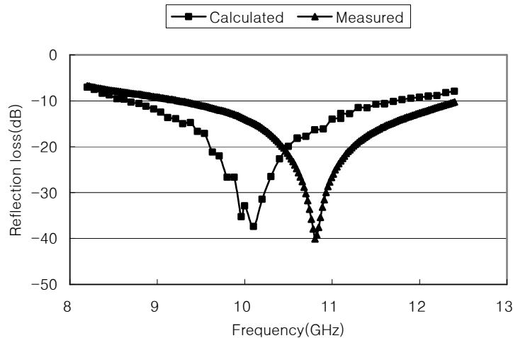
Fig. 5 Measured and calculated reflection loss of the optimal absorbing structure
