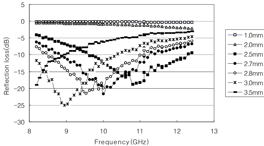
Fig. 3 Simulated reflection loss of glass fabric/epoxy composites with 6% carbon black (CB6)
