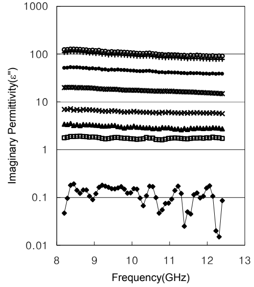
Fig. 2 Imaginary part of permittivity vs carbon black content
