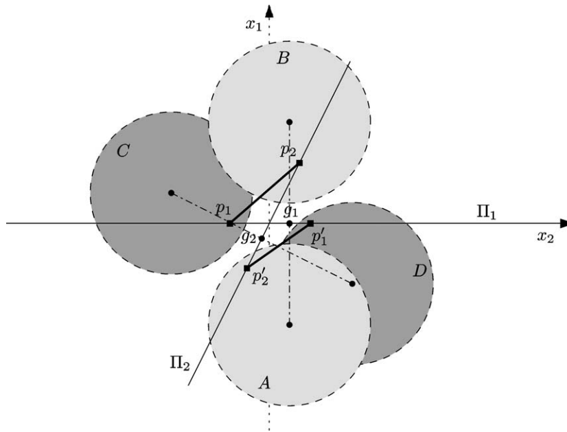
Fig. 5. The two hyperplanes define four quadrants.
