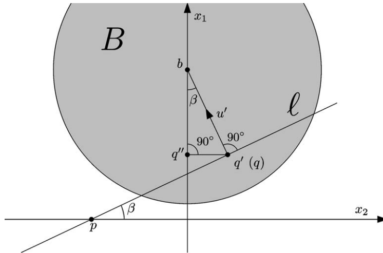
Fig. 4. The configuration projected on the x_1x_2 -plane.
