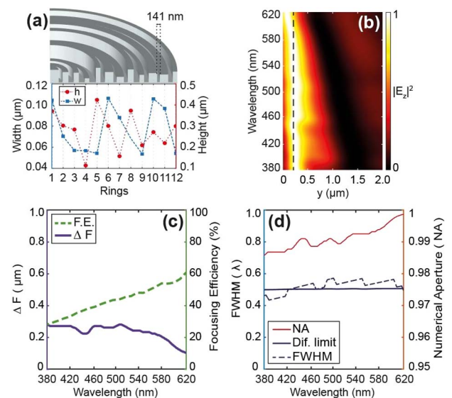
Fig. 6. (a) Quarter-cross sectional view of the nano-scaled lens with the plot of height and width for each zone. (b) Map of cross-sectional intensity profiles on optical axis, (c) plots of both \Delta F and focusing efficiency, and (d) graphs of both NA and FWHM values with respect to operating wavelengths of 380 and 620 nm.
