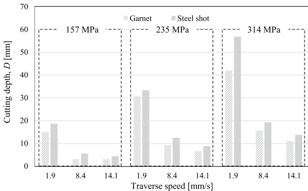
Fig. 5 Effects of the traverse speed on the cutting depth
