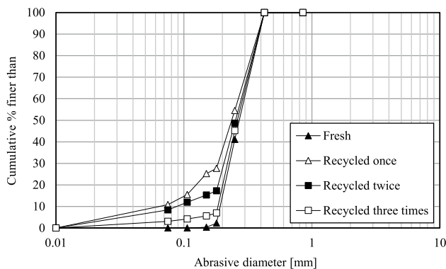
Fig. 14 Particle-size distribution
