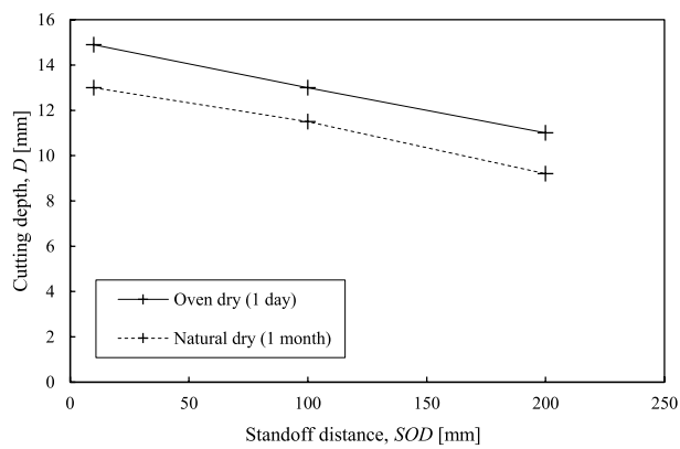
(a) Depth of cut as a function of the standoff distance
