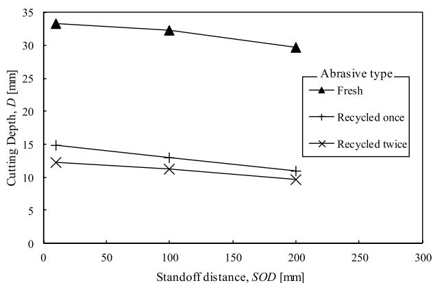
Fig. 11 Effects of the recycling times on the cutting depth using fresh steel and recycled steel shot
