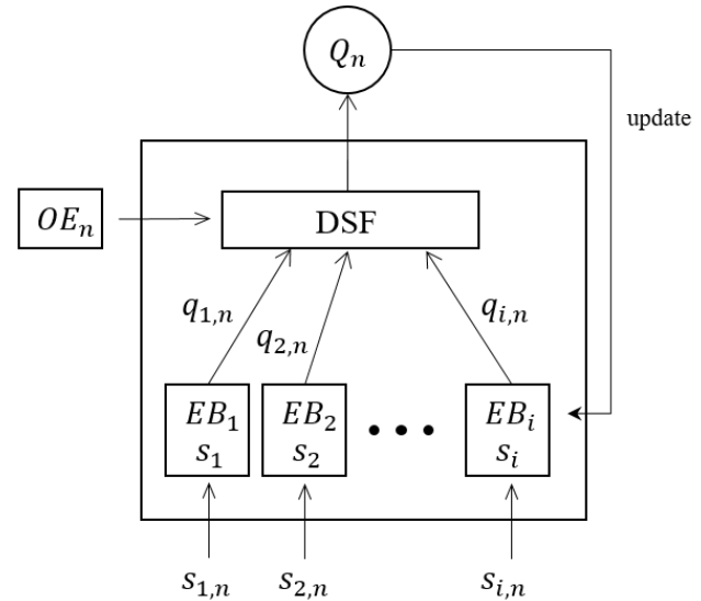
Fig. 10. DSF process for handling outliers.
