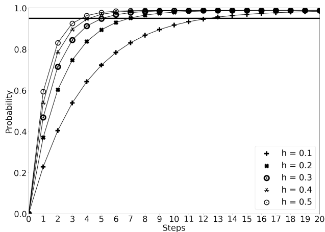
Fig. 9. Error correction convergence with different h values.
