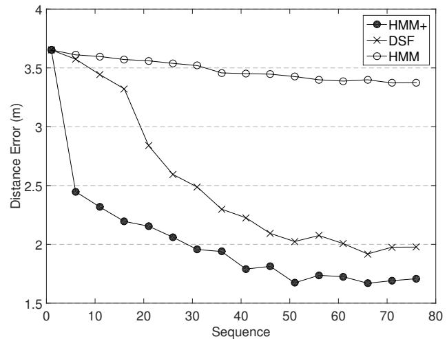
Fig. 17. Comparison of distance-, heading- and barometer-dependent tracking.
