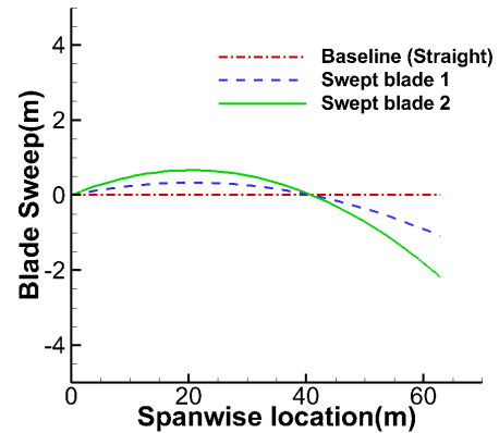
(a) Blade sweep
