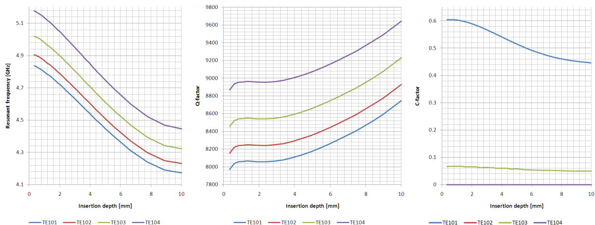
Figure 5: Result of a numerical simulation of the tunable waveguide structure. From left to right: Resonant frequency, unloaded Q -factor and the geometric C -factor are plotted vs. the insertion depth of the dielectric rods.
