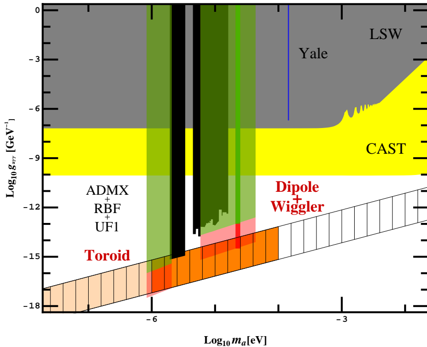
Figure 1: Existing bounds for axion-like particles [15–21]. Compilation adapted from [22]. The true QCD axion-region is marked as the hatched band. In the orange region axions are a natural candidate for dark matter. In the lighter shaded orange area axions can still be dark matter but with decreasing mass this requires an increasing amount of finetuning. Axion-like particles can be dark matter in a large part of the so far untested parameter space (cf. [12, 13]). The right green (red) regions are the conservatively (realistically) expected sensitivity of a dipole or wiggler search for axion-like particle dark matter. The more solidly shaded part in the middle of this region corresponds to the region probed by a single cavity with parameters as discussed in Sect. 2.1. The left green/red region shows the masses and couplings that could be probed in a setup with a toroidal magnet.
