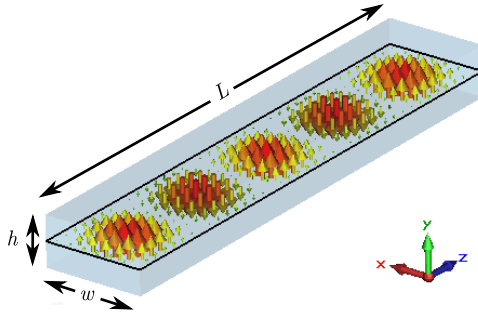
Figure 2: Electric field distribution of the TE_{105} mode in a rectangular waveguide.
