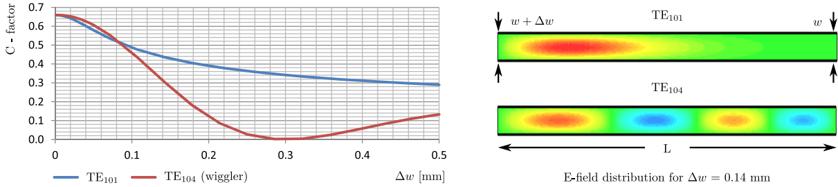
Figure 3: Left: Geometric form factor according to Eq. 2.6 as a function of \Delta w . Right: Snapshot of the electric field in the cavity, showing mode localization for \Delta w = 0.14 mm. The dimensions of the cavity are w=30 , h=20 , l=1500 mm. Note that the field plots are not to scale.
