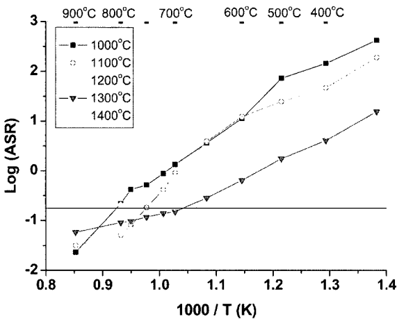
Fig. 8. Sintering temperature dependence of the ASR in air.
