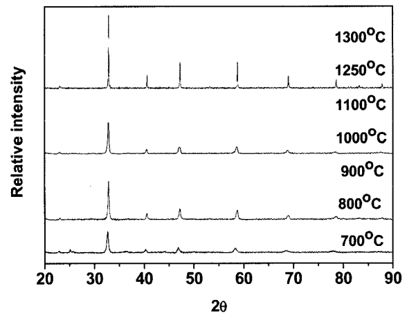
Fig. 2. XRD patterns of Pr_{0.3}Sr_{0.7}Co_{0.3}Fe_{0.7}O_3 with variable calcination temperature.
