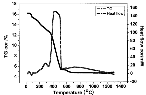
Fig. 1. TG-DSC curves for Pr_{0.3}Sr_{0.7}Co_{0.3}Fe_{0.7}O_3 .
