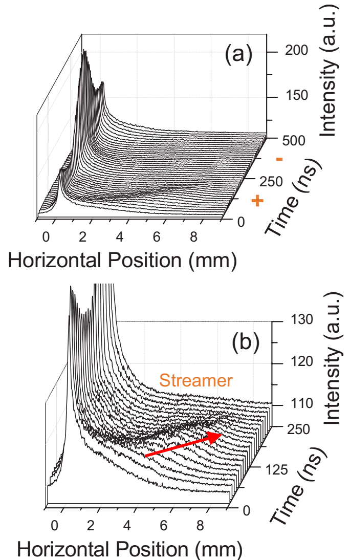
FIG. 2. (Color online) 3D plot for a time-resolved image of the dual frequency plasma and (b) zoom in of the plot for the positive period at a total P_{in}=150 W (75 W each).
