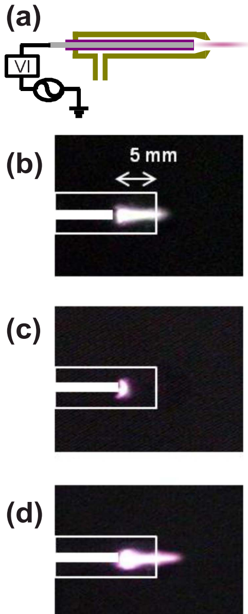
FIG. 1. (Color online) (a) Schematic of the plasma source and plasma images for single frequency of (b) 2 MHz and (c) 13.56 MHz, both at P_{in}=75 W, and for dual frequency of (d) 2 MHz+13.56 MHz at a total P_{in}=150 W (75 W each).
