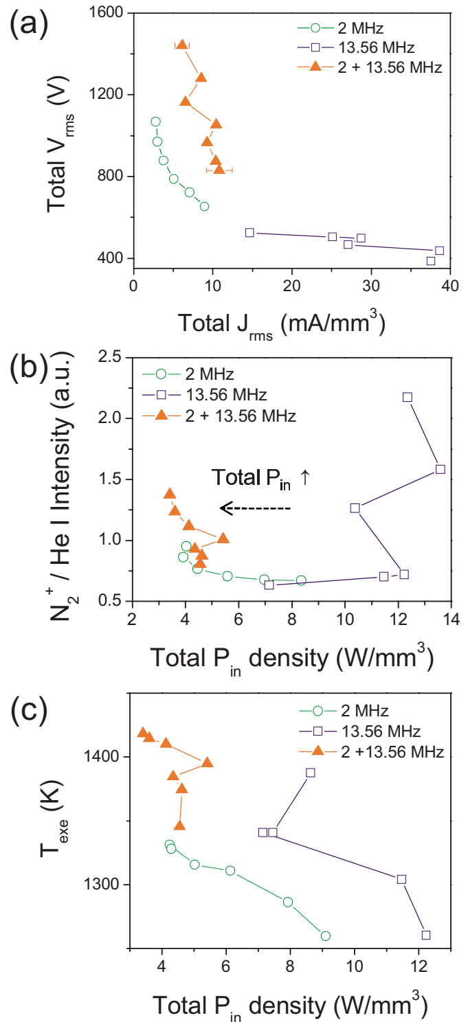
FIG. 3. (Color online) (a) Total volume current density vs voltage curve. (b) \text{N}_2^+ (391.4 nm) intensity normalized to He I (706.5 nm) for total volume power density. The total P_{\text{in}} density was decreased as the total P_{\text{in}} was increased due to the discharge volume expansion. The dotted arrow in the plot shows the total P_{\text{in}} increase direction. (c) T_{\text{exe}} vs total volume power density. For the dual frequency case, the 2 MHz P_{\text{in}} was varied from 10 to 100 W while the 13.56 MHz P_{\text{in}} was fixed at 75 W.
