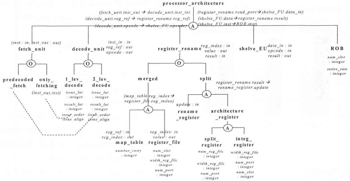
Fig. 2 Design Space of Superscalar Processor Architecture
