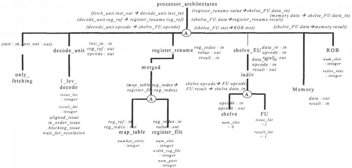
Fig. 3 Pruned Design Space
