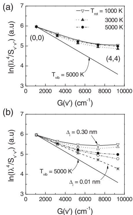
FIG. 3. (a) Difference in the Boltzmann plot caused by different T_{rot} values ( T_{vib}=5000 K (—) and \Delta_i=0.01 nm). (b) Difference in the Boltzmann plot due to different \Delta_i values: \Delta_i=0.01 nm (—*—), 0.05 nm (—○—), 0.10 nm (—●—), 0.20 nm (—△—), and 0.30 nm (—▽—). The straight line indicates the Boltzmann plot for T_{vib}=5000 K without considering the instrumental broadening.
