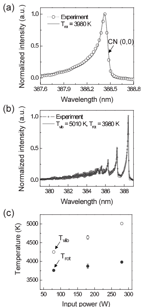
FIG. 6. (a) T_{rot} obtained by the comparison between the experimental result (—○—) and the synthetic spectrum (—) of CN (0,0) band is 3980 K. (b) Comparison of the whole CN spectra provides T_{vib} of 5010 K and T_{rot} of 3980 K at 280 W. (c) As the input power is increased, both T_{vib} and T_{rot} are also increased from 4250 to 5010 K and from 3760 to 3980 K, respectively. \Delta\lambda=0.065 nm.
