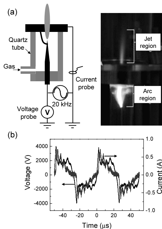
FIG. 4. Schematic illustration of the (a) experimental setup for atmospheric pressure arc discharge, and (b) voltage and current oscillogram during the discharge.
