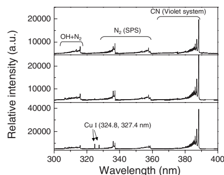
FIG. 5. Emission spectra at various input power: 80, 180, and 280 W. Due to the mixed gas of CH_4 , N_2 , and O_2 , and air impurities, the OH, N_2 , and CN molecular spectra are observed.
