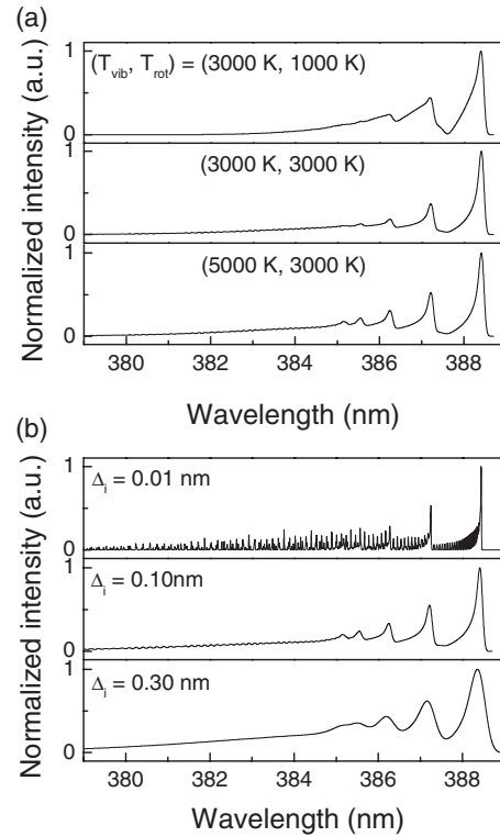
FIG. 2. (a) The synthetic CN (violet system) spectra at various T_{\text{vib}} and T_{\text{rot}} at fixed \Delta_i=0.1 nm. (b) The synthetic CN (violet system) spectra at different \Delta_i from 0.01 to 0.30 nm ( T_{\text{vib}}=T_{\text{rot}}=5000 K).
