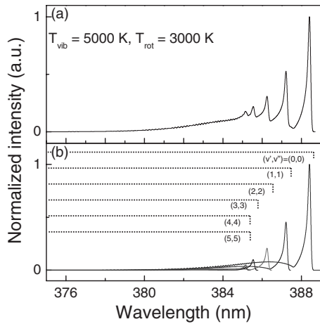
FIG. 1. (a) The synthetic CN (violet system) spectrum at T_{\text{vib}}=5000 K, T_{\text{rot}}=3000 K, and \Delta_i=0.10 nm. (b) Each rotational band for each vibrational state from (0,0) to (5,5).
