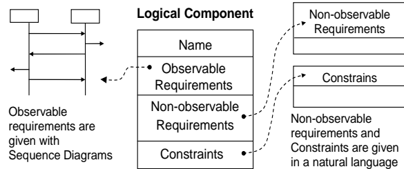
Figure 6. ALFRéD specification of a logical component
