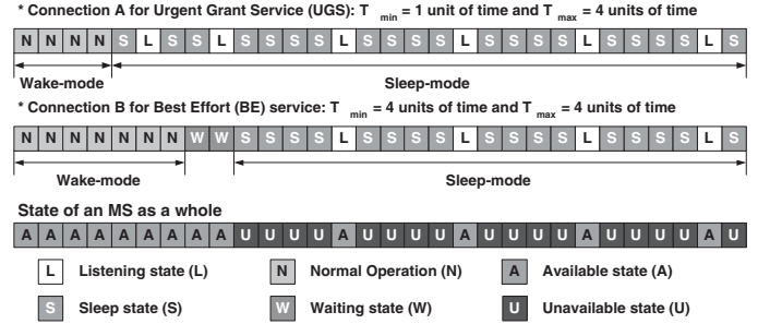
Fig. 2. Example of the behavior of an MS with sleep-mode operations for two connections under the new SPSM.
