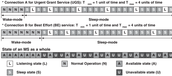
Fig. 1. Example of the behavior of an MS with sleep-mode operations for two connections under the standard PSM (the size of listening interval = 1 unit of time ( U )) ([1], Figure 130a).
