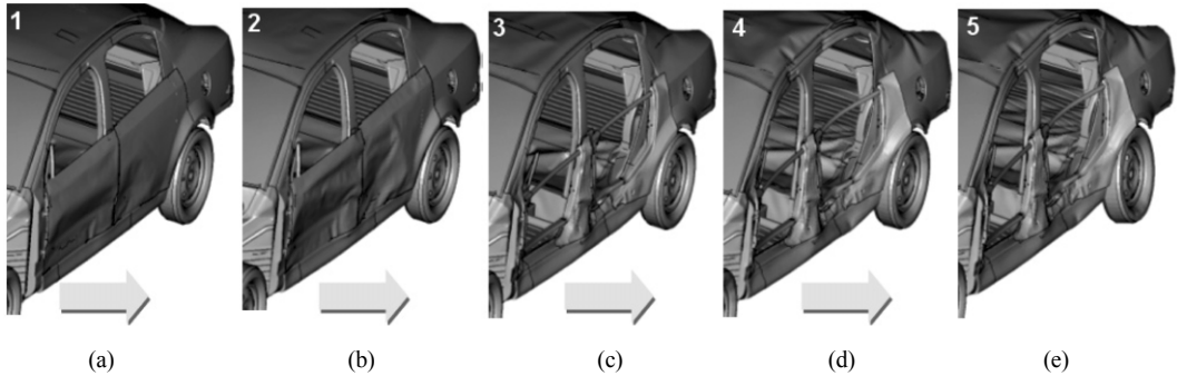
Fig. 11 Subsequent deformation mechanism with AHSS: (a) 0.007sec; (b) 0.011 sec; (c) 0.016 sec; (d) 0.03 sec; (e) 0.047 sec
