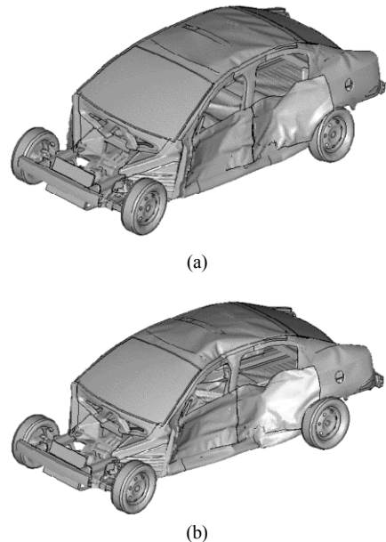
Fig. 8 Deformed shapes of the vehicle for the crash analysis at time 0.06sec: (a) AHSS; (b) conventional steel
