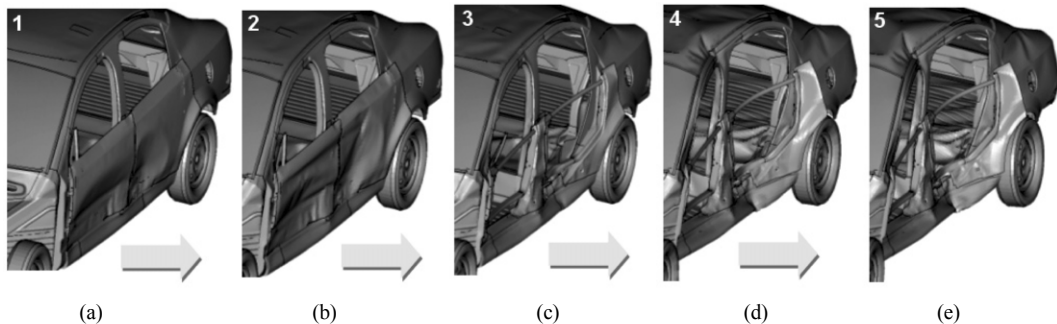
Fig. 12 Subsequent deformation mechanism with conventional steel: (a) 0.0088sec; (b) 0.0143 sec; (c) 0.02 sec; (d) 0.04 sec; (e) 0.06 sec
