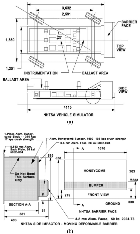
Fig. 1 Facility and equipment for SINCAP test procedure : (a) vehicle simulator; (b) side impactor- moving deformable barrier
