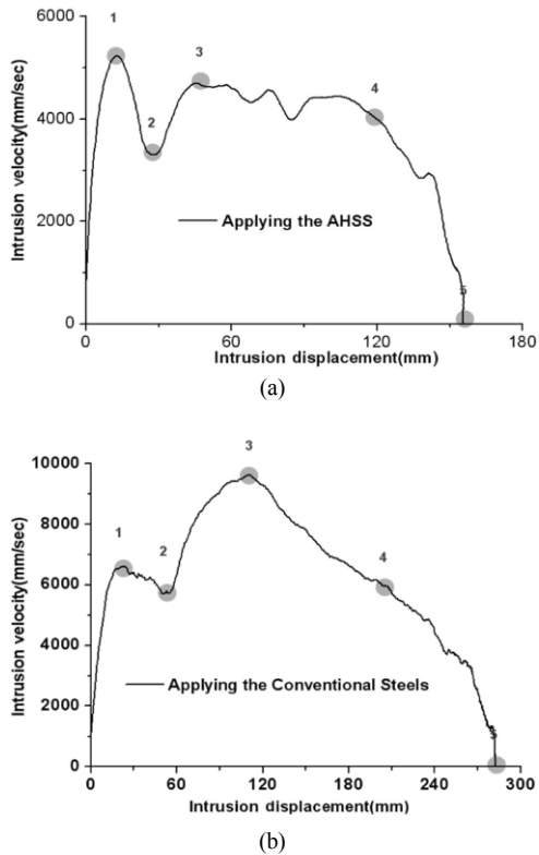
Fig. 10 Points of time at which the local minimum and local maximum velocity occurs: (a) AHSS; (b) conventional Steel
