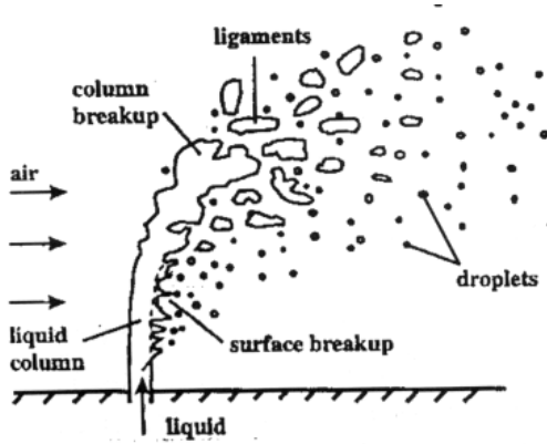
Fig. 1 Sketch of a typical liquid breakup process in crossflow ; reproduced from reference[8]
