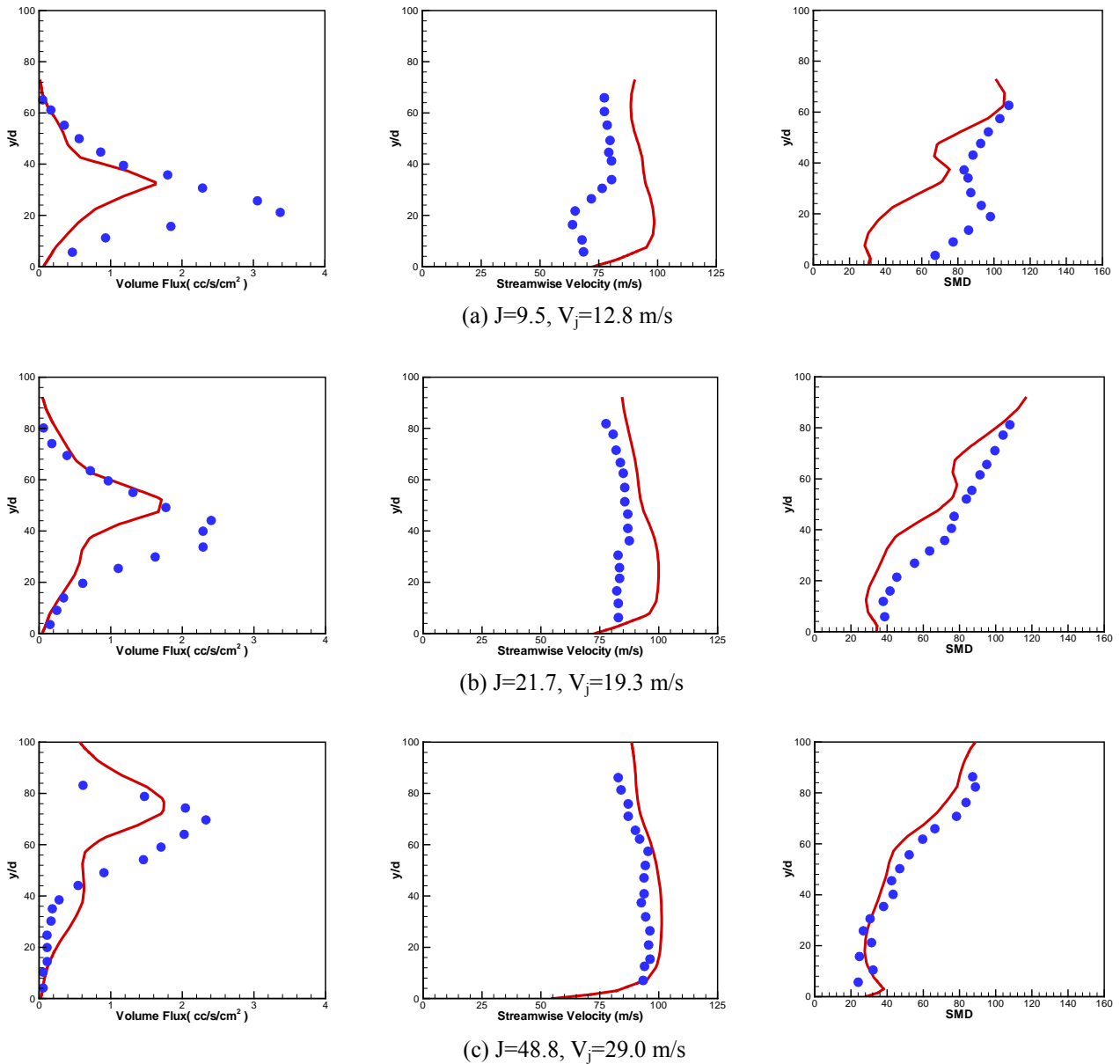
Fig. 5 Centerline profiles of droplet volume flux, streamwise velocity, and Sauter mean diameter ( ● ; experimental data[14], solid line ; calculation )
