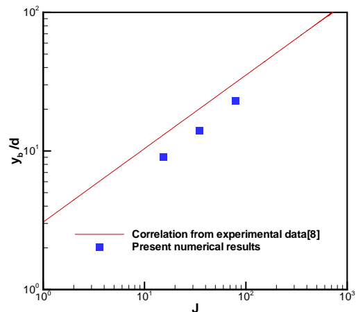
Fig. 4 Liquid column fracture heights
