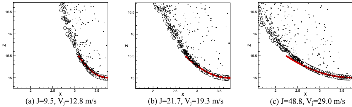
Fig. 3 Trajectories of liquid column (solid line ; correlation from experimental data)
