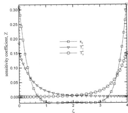
Fig. 6 Sensitivity coefficients for wall temperature and emissivity for the case 4
