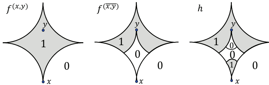
FIG. 3.1. Functions defined in the proof of Theorem 1.4: f^{(x,y)} , f^{(\bar{x},\bar{y})} , and h . Observe that f^{(x,y)}(x) = f^{(x,y)}(y) = 1 , f^{(\bar{x},\bar{y})}(x) = f^{(\bar{x},\bar{y})}(y) = 0 , h(x) = 1 , and h(y) = 0 .
