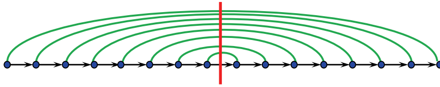
FIG. 4.2. An illustration for the proof of the lower bound on the size of a 2-TC-spanner for the line.
