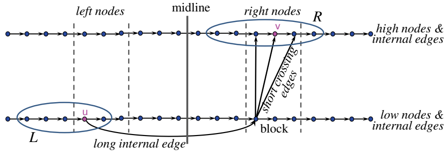
FIG. 4.4. An illustration of the first stage in the proof of Lemma 4.5.
