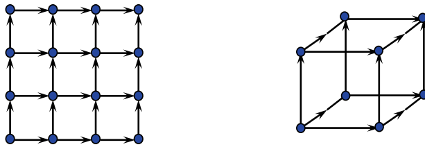
FIG. 1.2. Examples of hypergrids: \mathcal{H}_4^2 (left) and \mathcal{H}_3 (right). All edges are directed toward vertices with larger coordinates.
