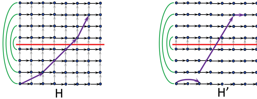
FIG. 4.5. An illustration for the proof of Lemma 4.6: an example transformation from H to H' . Arches to the left of each panel connect matched lines.
