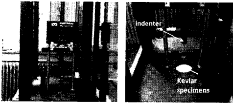
Fig. 2 Stab resistance test setup.
