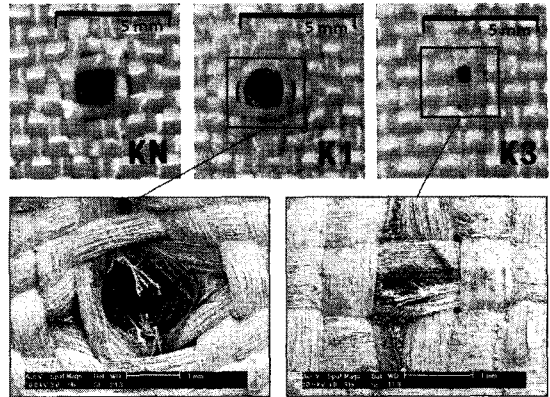
Fig. 8 Photographs and SEM images of the rear surface of the first layer at n=2.527\text{kg} and h=0.2\text{m} .
