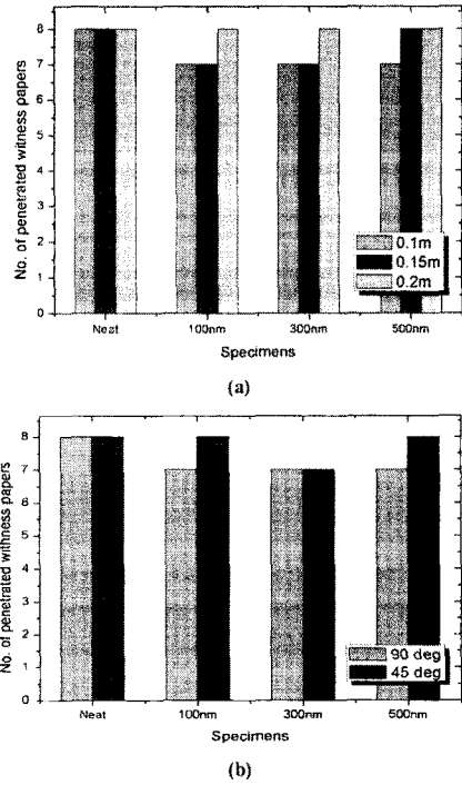
Fig. 14 Number of penetrated papers after knife drop tests (a) perpendicular blade orientation to woven direction at different drop height (b) different blade orientation to woven direction at h=0.1m, 2.47J
