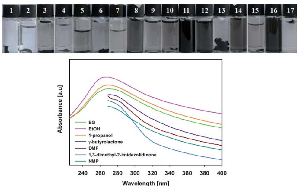
Fig. 1 (a) Photographs of reduced graphene dispersed in water and 16 organic solvents via 5 h sonication. The photographs were taken 1 month after the preparation of the reduced graphene dispersion. (b) UV-Vis absorption spectra of reduced graphene dispersed in good solvents. The spectra of NMP, 1,3-dimethyl-2-imidazolidinone, DMF, and \gamma -butyrolactone are only shown in the wavelength range from 269 nm to 400 nm due to compensation for their strong absorption at <269 nm.
