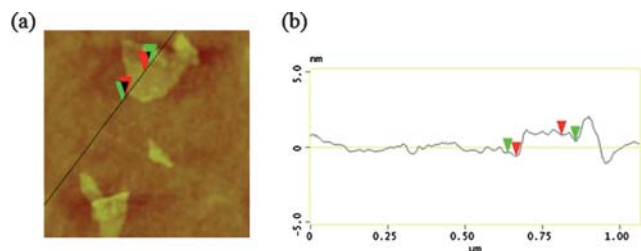
Fig. 2 (a) An AFM image ( 1\ \mu\text{m} \times 1\ \mu\text{m} ) of isolated reduced graphene sheets deposited onto an Si wafer from dispersion in 1,3-dimethyl-2-imidazolidinone, (b) a thickness profile of graphene sheets marked by the black line in (a), where the height differences are 1.77 nm between the two black arrows, 0.91 nm between the two red arrows and 1.24 nm between the two green arrows, respectively.
