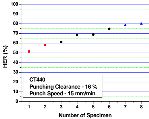
Fig. 7 hole expansion ratio of CT440 with 16% of punching clearance and 15 mm/min of punch speed
