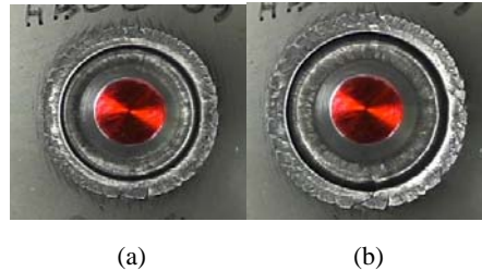
Fig. 2 pictures of the edge of the hole manufactured by punching for FB590: (a) 32 sec; (b) final fracture
