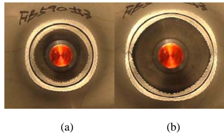
Fig. 3 Pictures of the edge of the hole manufactured by machining for FB590: (a) 120 sec; (b) final fracture
